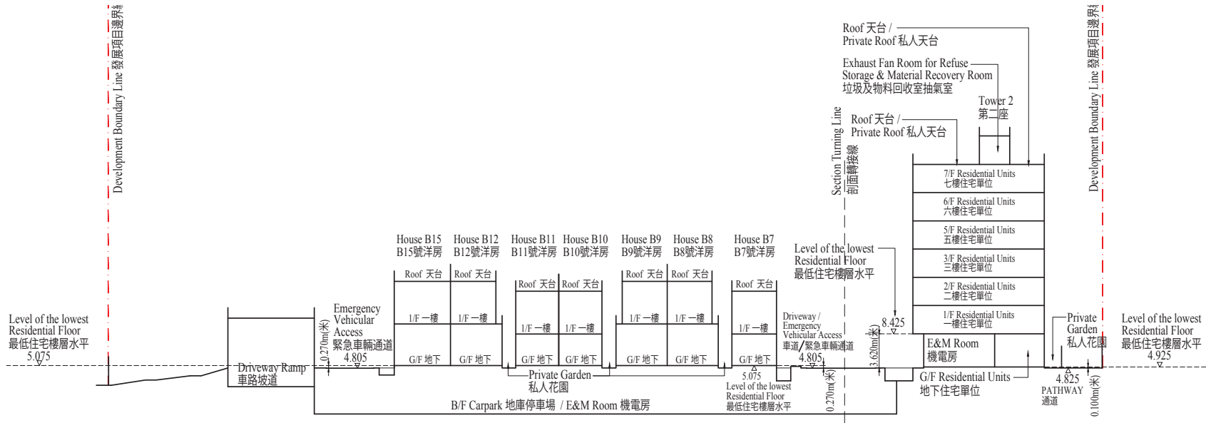
橫截面圖 K-K CROSS-SECTION PLAN K-K
